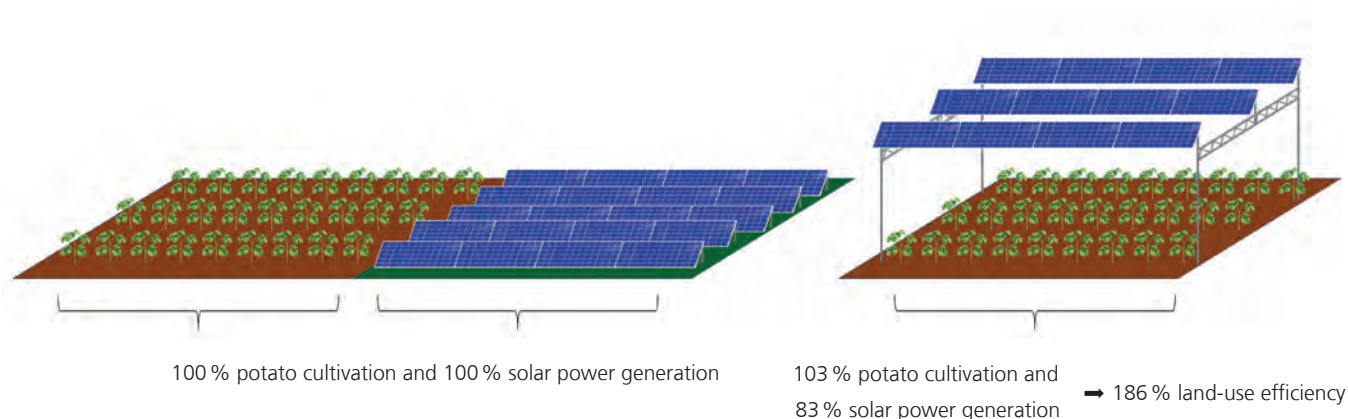
Fig. 15: The dual use of land for agrivoltaics and potato growing increased land-use efficiency on the Heggelbach test site to 186 percent © Fraunhofer ISE
